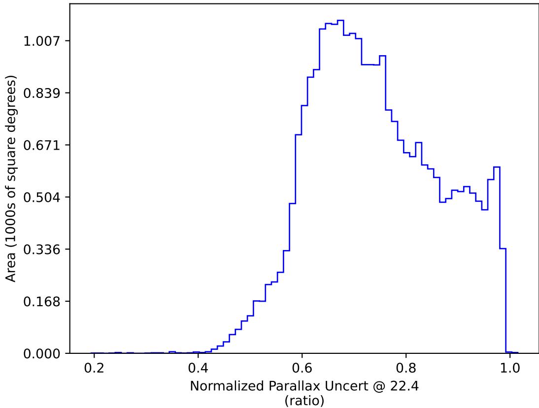
too_combined_s0.5_v3.4_10yrs All sky: Normalized Parallax Uncert @ 22.4
