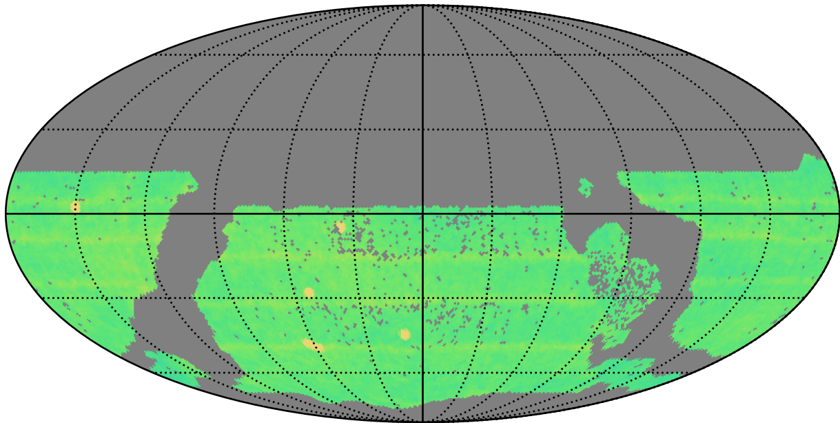
too_combined_s0.5_v3.4_10yrs WFD all bands: N Unique Nights
