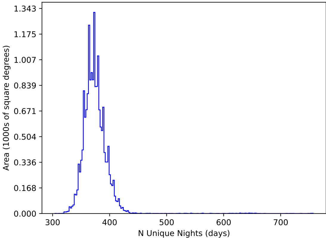
too_combined_s0.5_v3.4_10yrs WFD all bands: N Unique Nights
