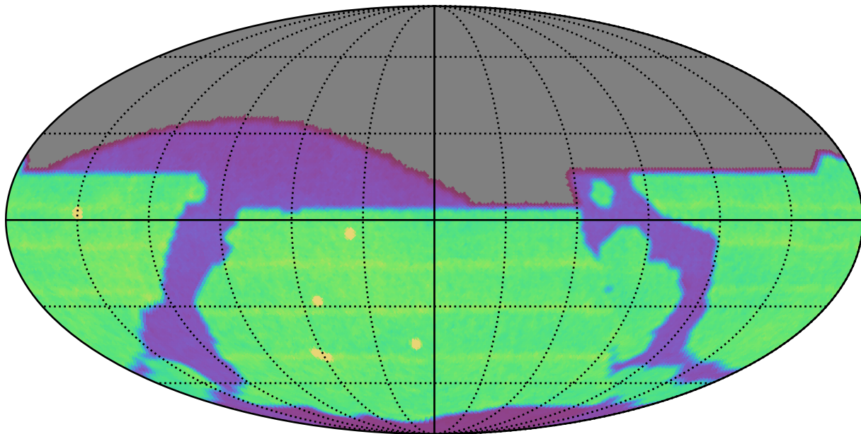
too_combined_s0.5_v3.4_10yrs All sky all bands: N Unique Nights
