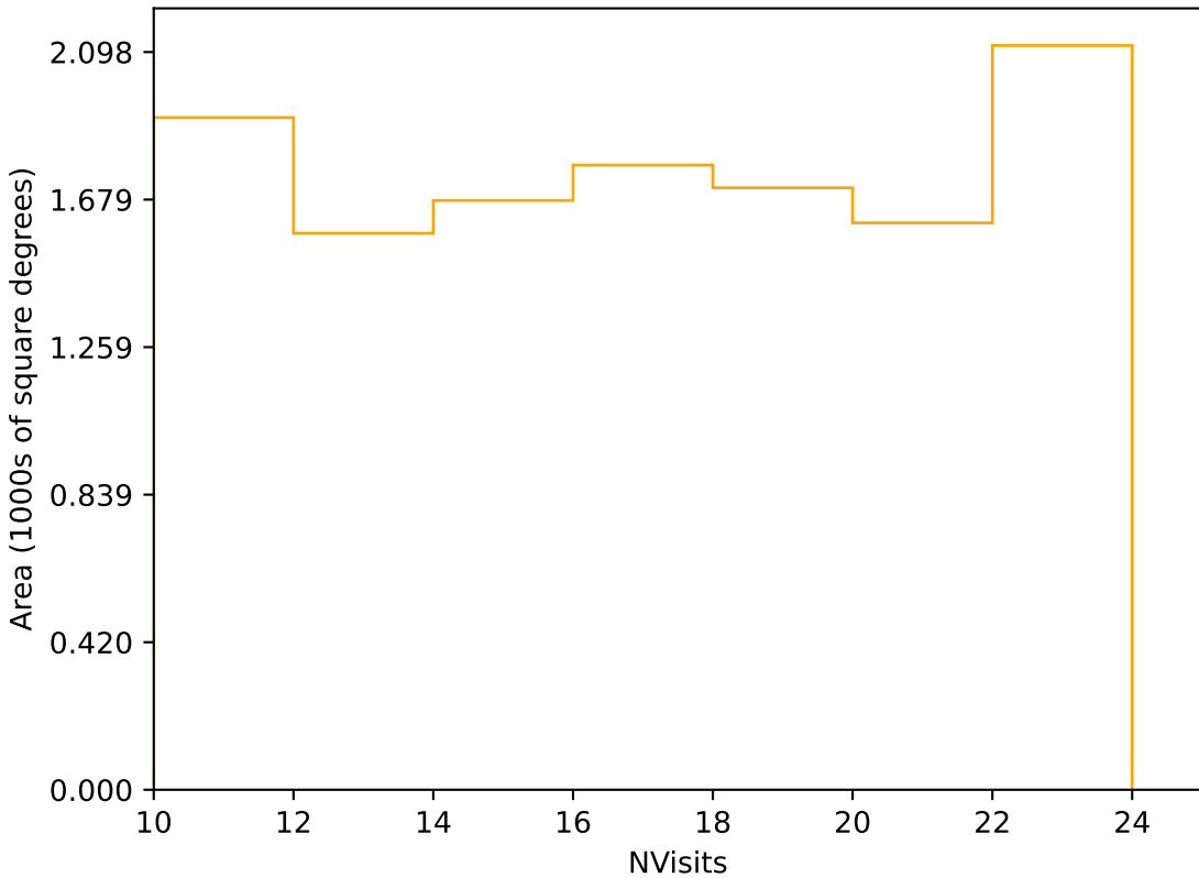
too_combined_s0.5_v3.4_10yrs Yr 3-4 r band: NVisits
