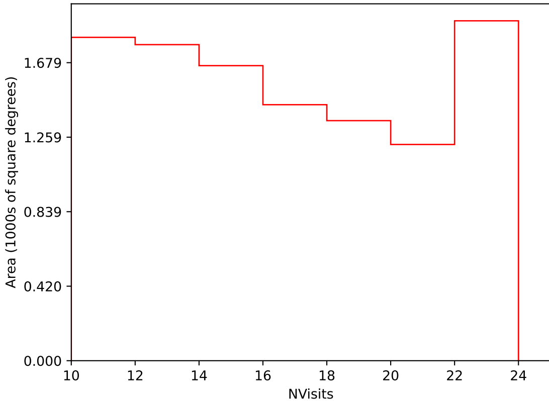
too_combined_s0.5_v3.4_10yrs Yr 3-4 i band: NVisits
