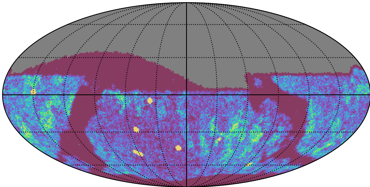
too_combined_s0.5_v3.4_10yrs Yr 1 z band: NVisits
