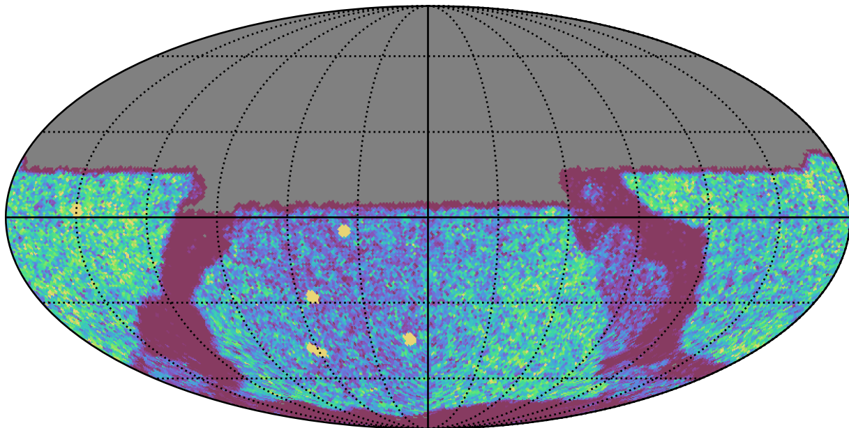
too_combined_s0.5_v3.4_10yrs Yr 1 y band: NVisits
