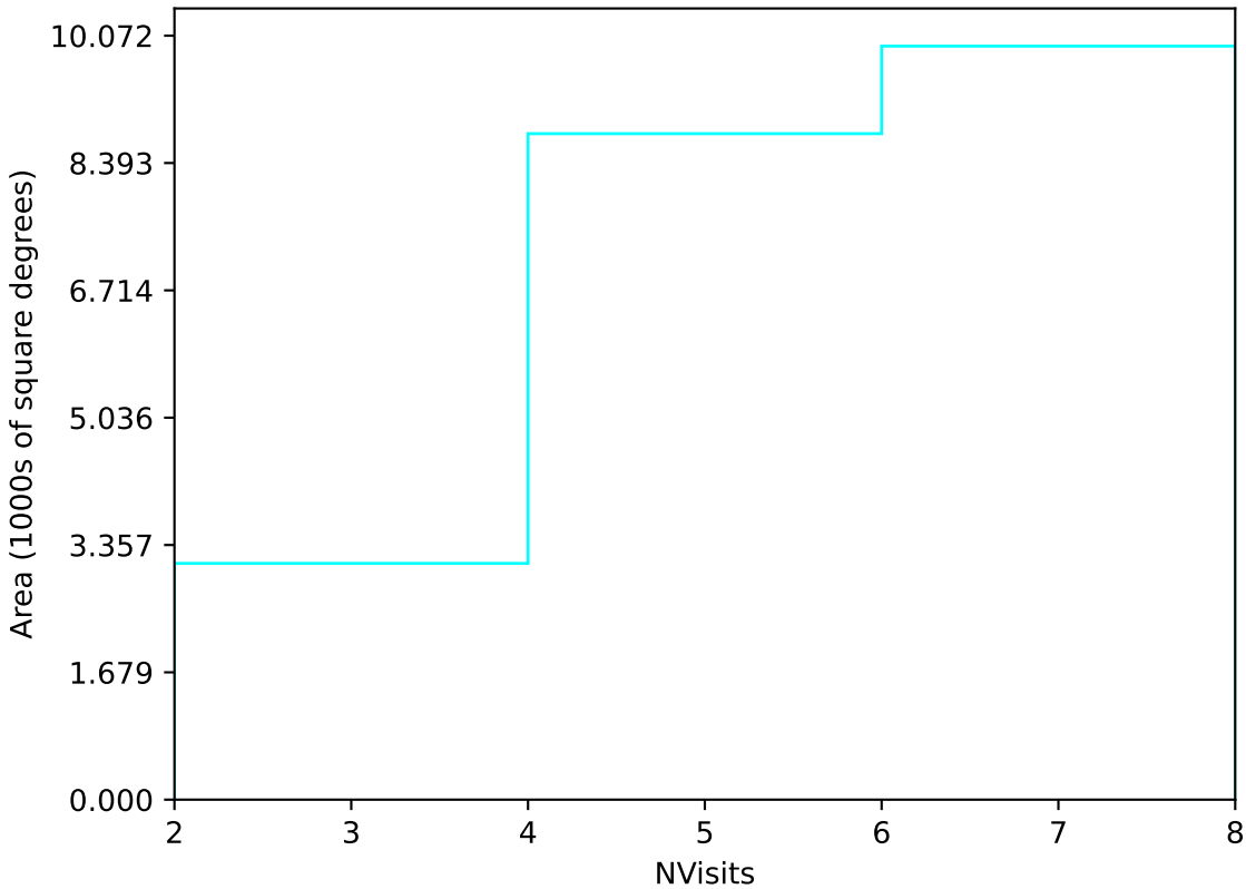
too_combined_s0.5_v3.4_10yrs Yr 1 u band: NVisits
