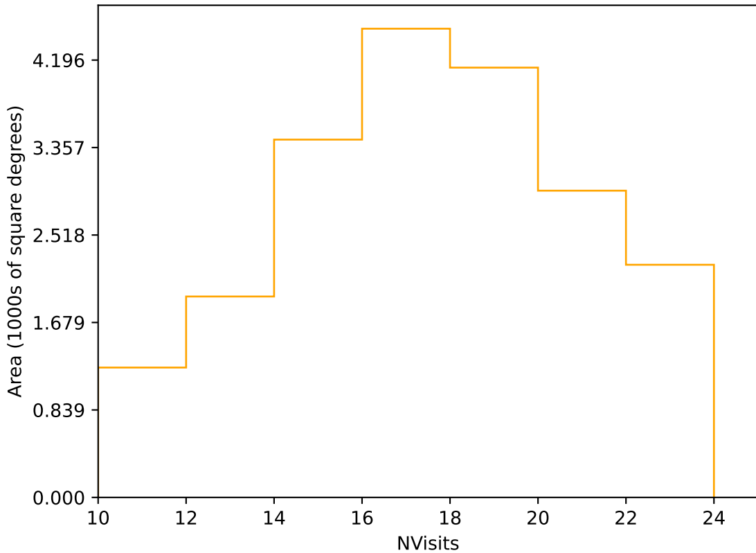
too_combined_s0.5_v3.4_10yrs Yr 1 r band: NVisits
