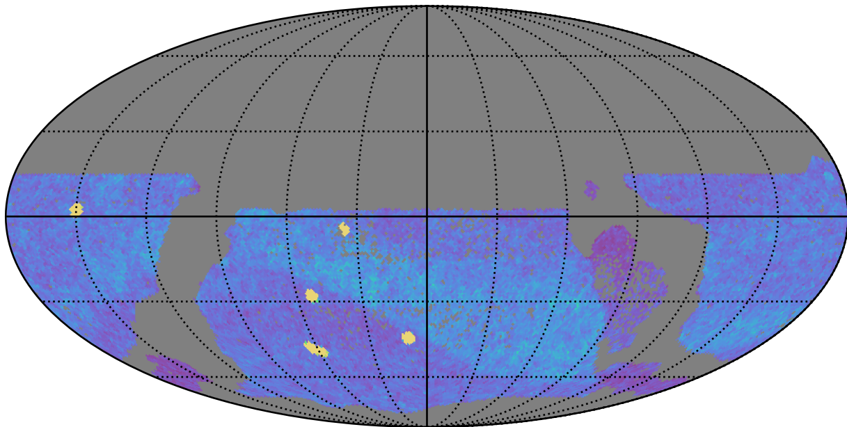
too_combined_s0.5_v3.4_10yrs WFD z band: NVisits
