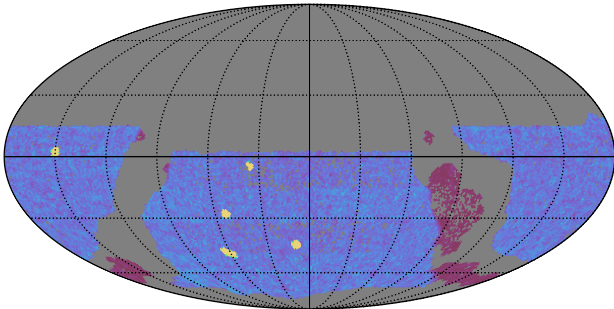
too_combined_s0.5_v3.4_10yrs WFD y band: NVisits
