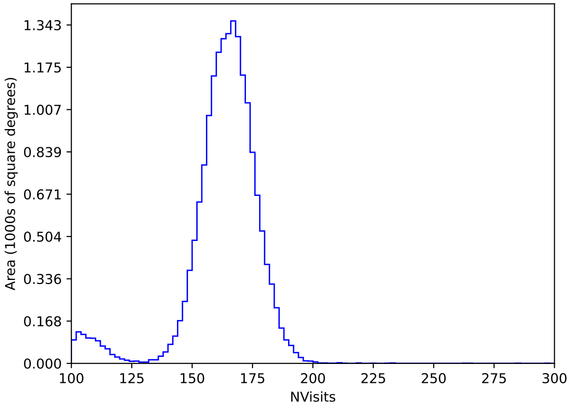
too_combined_s0.5_v3.4_10yrs WFD y band: NVisits
