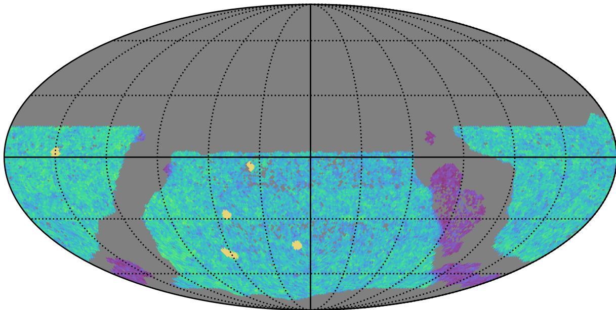
too_combined_s0.5_v3.4_10yrs WFD u band: NVisits
