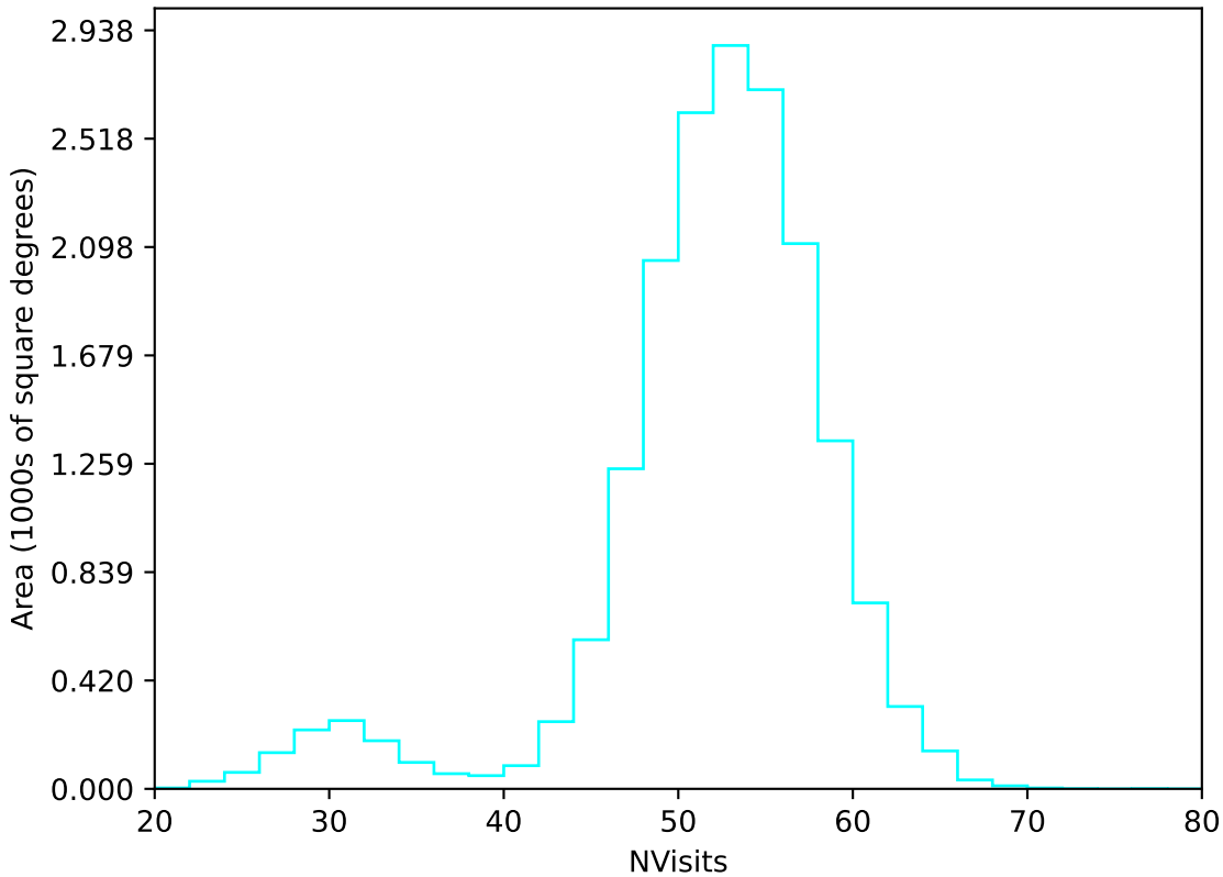
too_combined_s0.5_v3.4_10yrs WFD u band: NVisits
