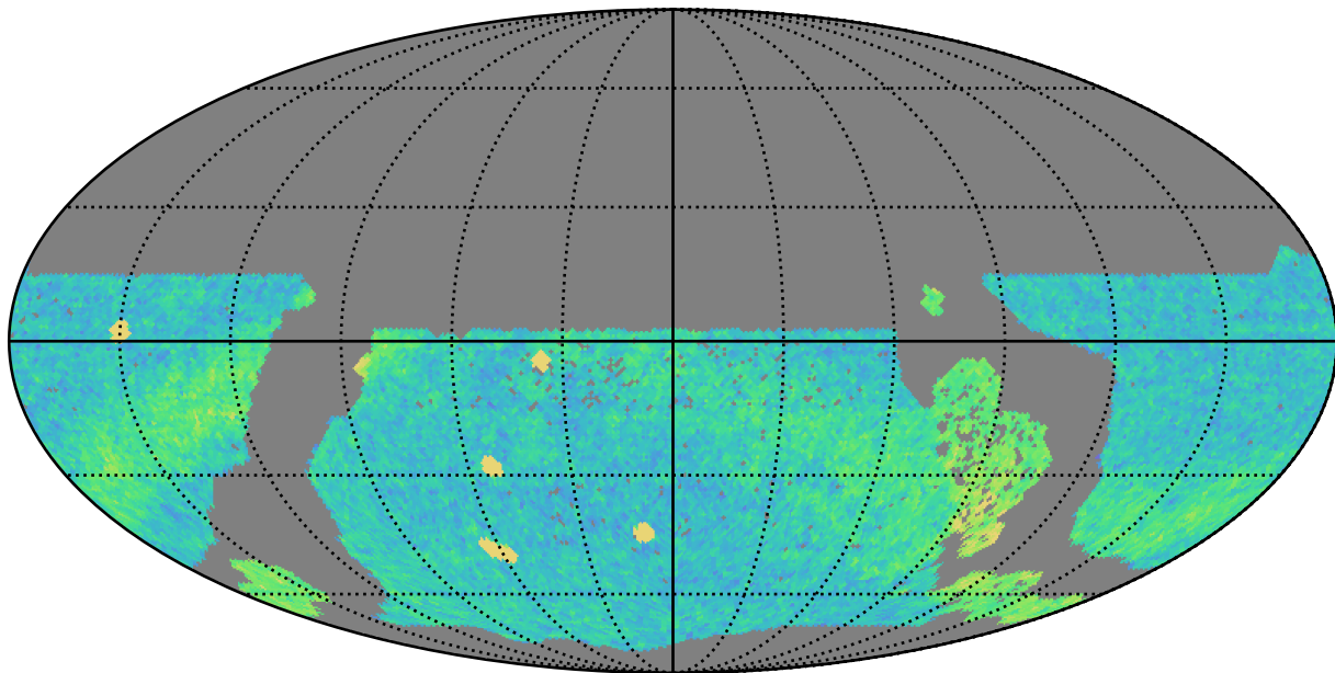
too_combined_s0.5_v3.4_10yrs WFD r band: NVisits
