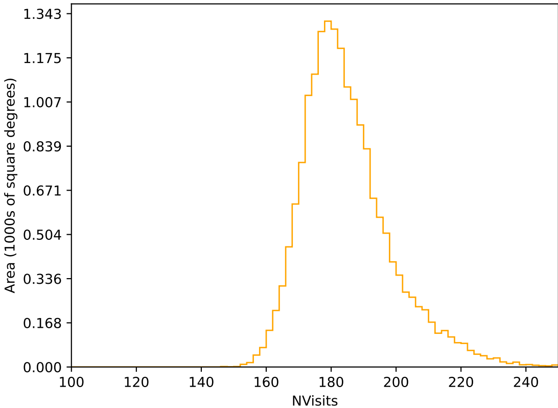
too_combined_s0.5_v3.4_10yrs WFD r band: NVisits
