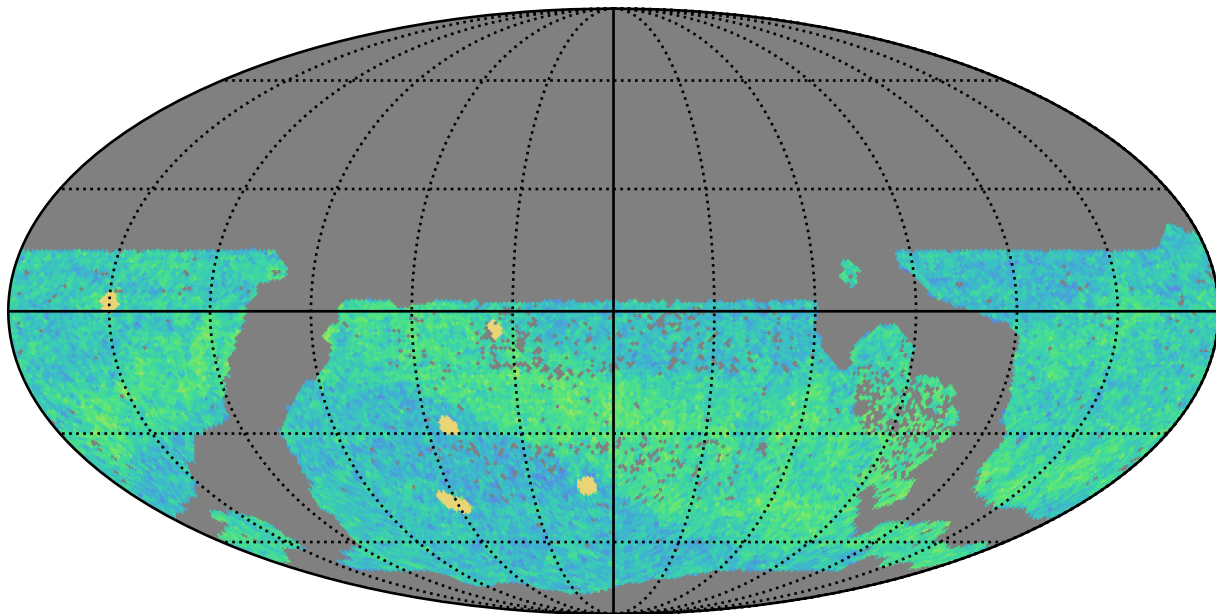
too_combined_s0.5_v3.4_10yrs WFD i band: NVisits
