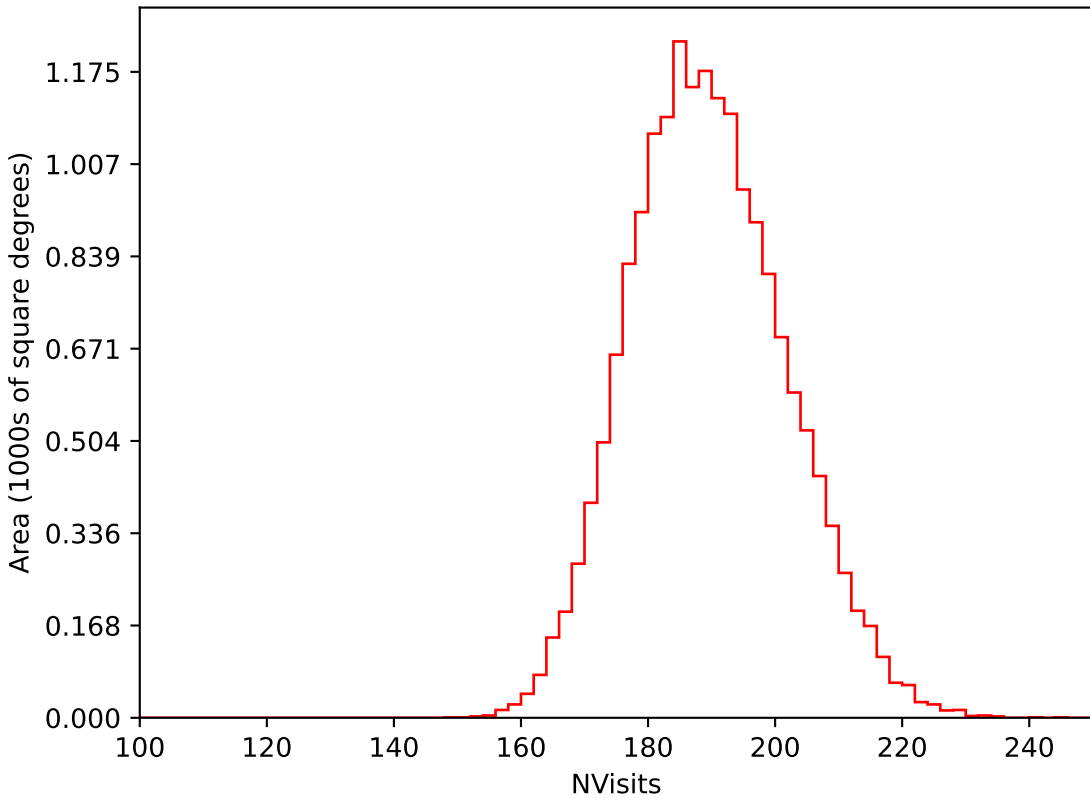
too_combined_s0.5_v3.4_10yrs WFD i band: NVisits
