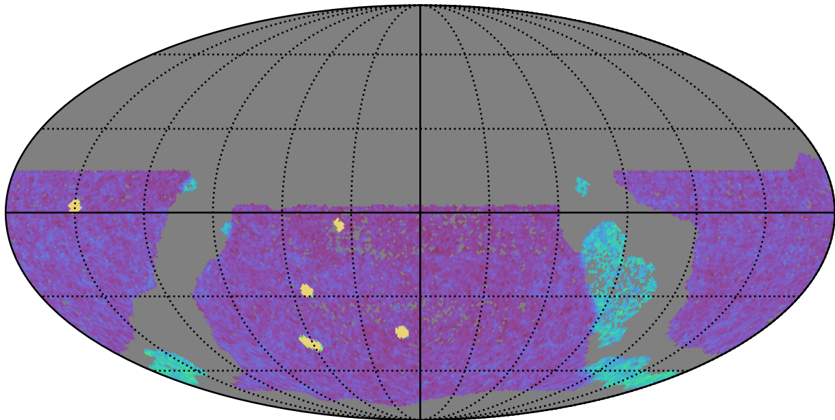
too_combined_s0.5_v3.4_10yrs WFD g band: NVisits
