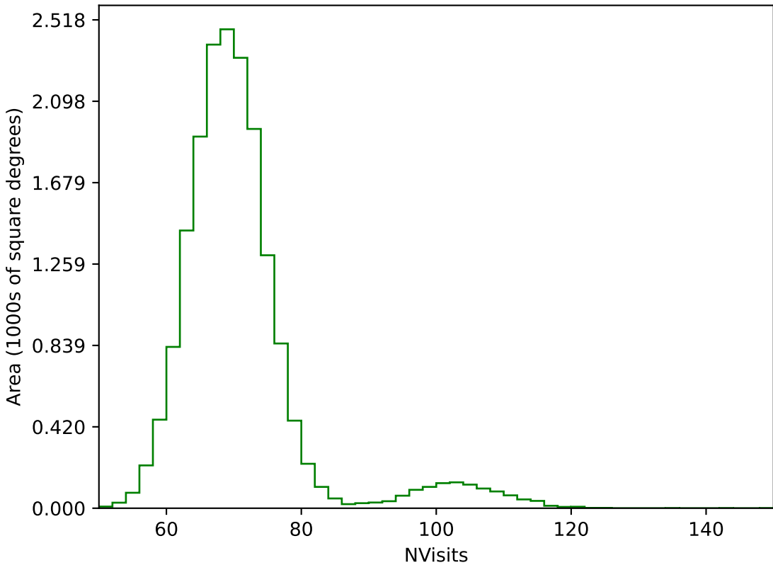
too_combined_s0.5_v3.4_10yrs WFD g band: NVisits
