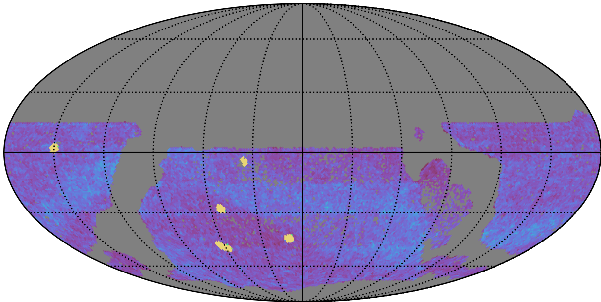
too_combined_s0.5_v3.4_10yrs WFD all bands: NVisits
