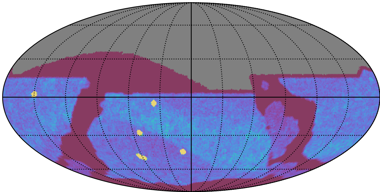
too_combined_s0.5_v3.4_10yrs All sky z band: NVisits
