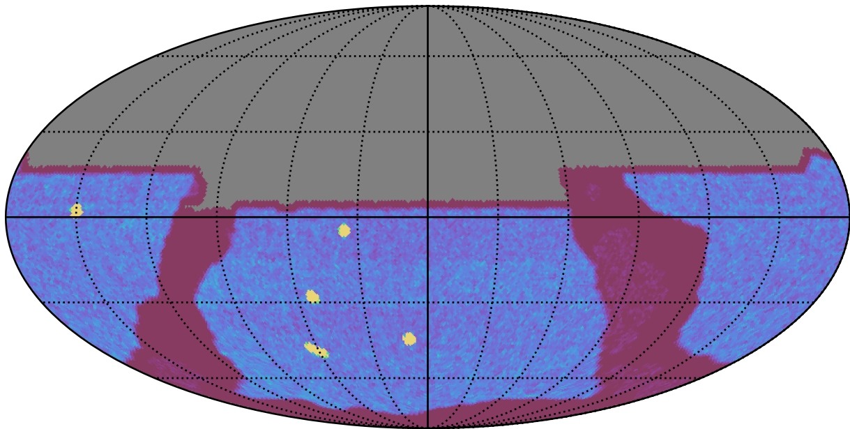
too_combined_s0.5_v3.4_10yrs All sky y band: NVisits
