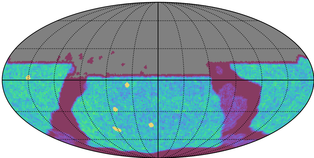
too_combined_s0.5_v3.4_10yrs All sky u band: NVisits
