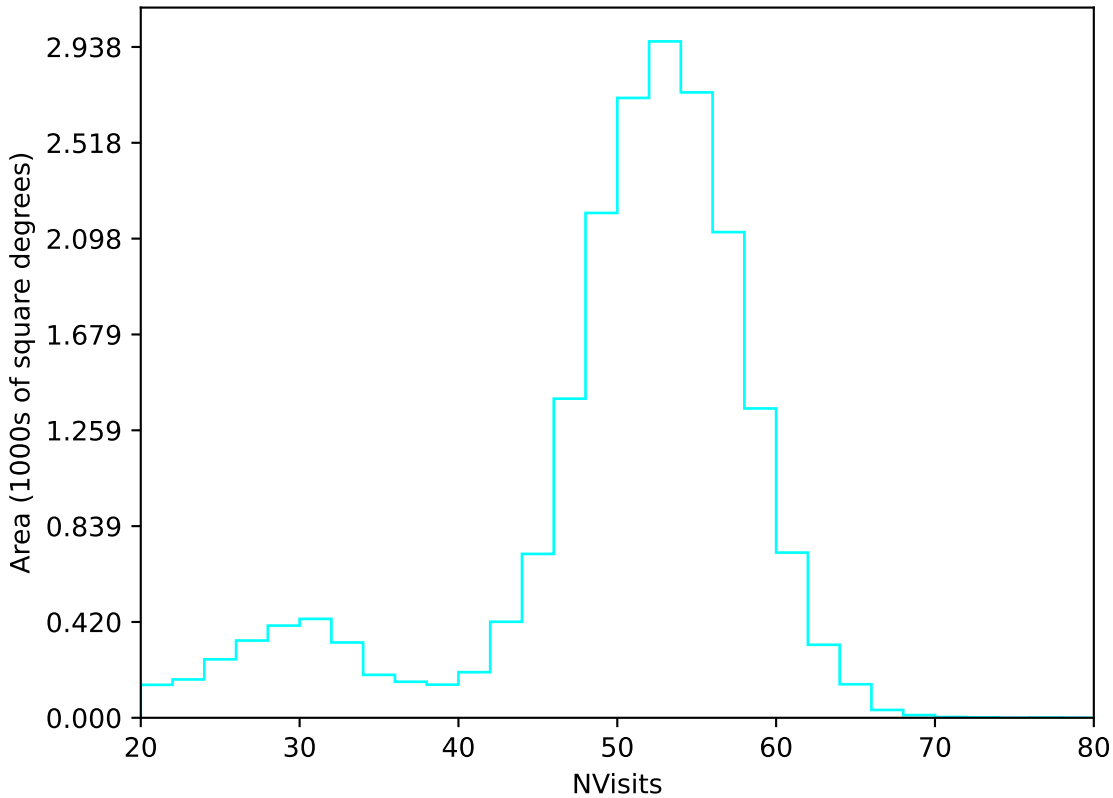
too_combined_s0.5_v3.4_10yrs All sky u band: NVisits
