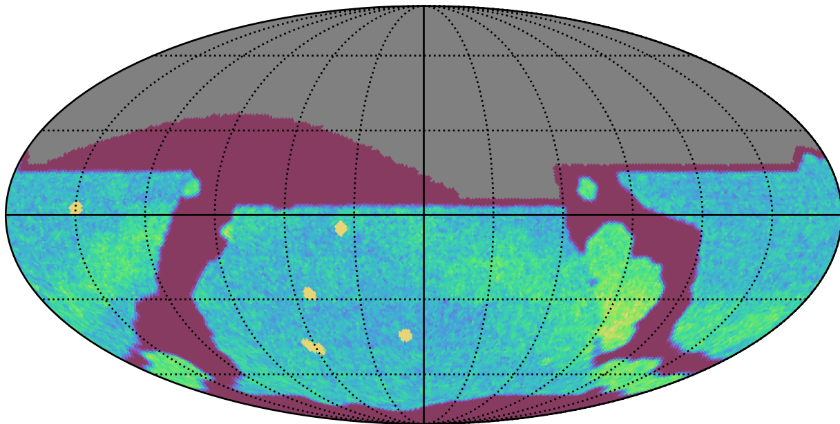
too_combined_s0.5_v3.4_10yrs All sky r band: NVisits
