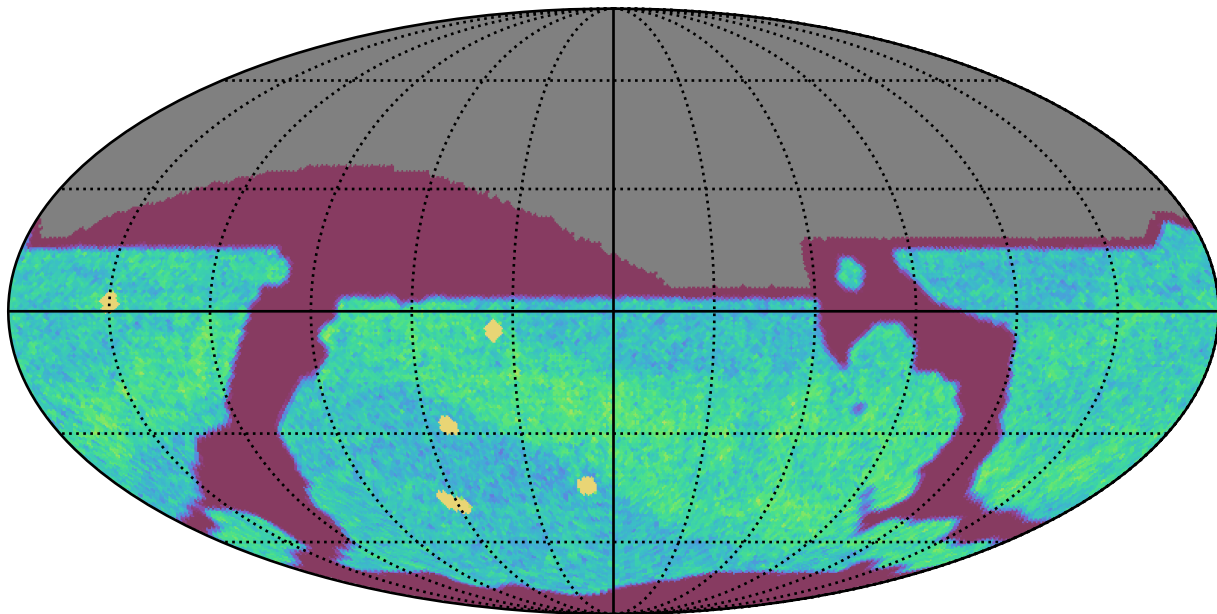
too_combined_s0.5_v3.4_10yrs All sky i band: NVisits
