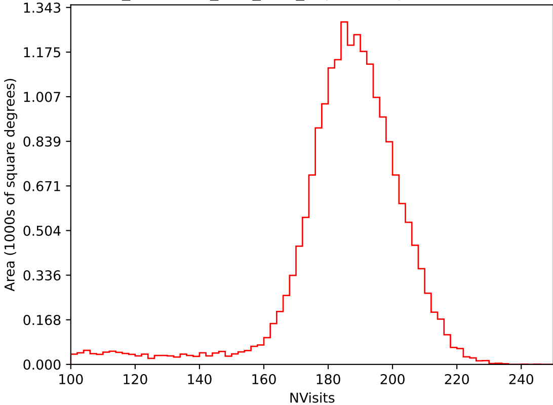
too_combined_s0.5_v3.4_10yrs All sky i band: NVisits
