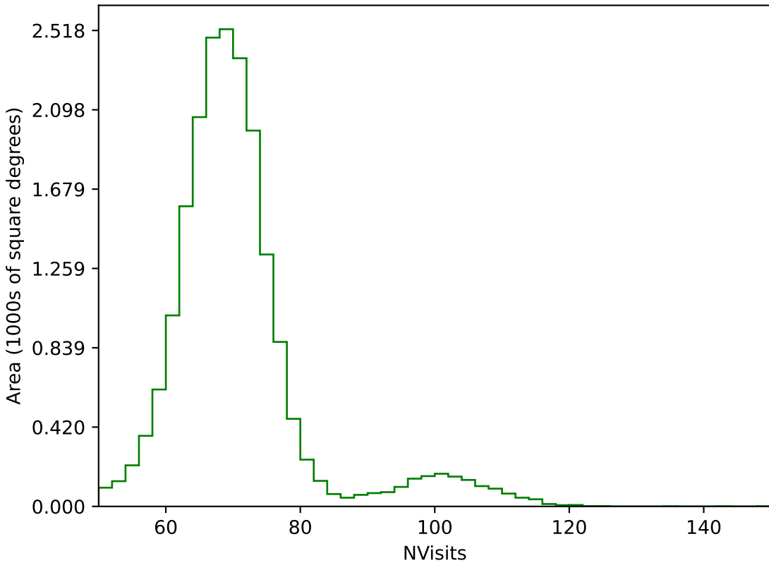
too_combined_s0.5_v3.4_10yrs All sky g band: NVisits
