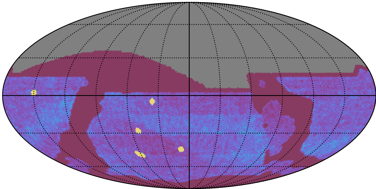
too_combined_s0.5_v3.4_10yrs All sky all bands: NVisits
