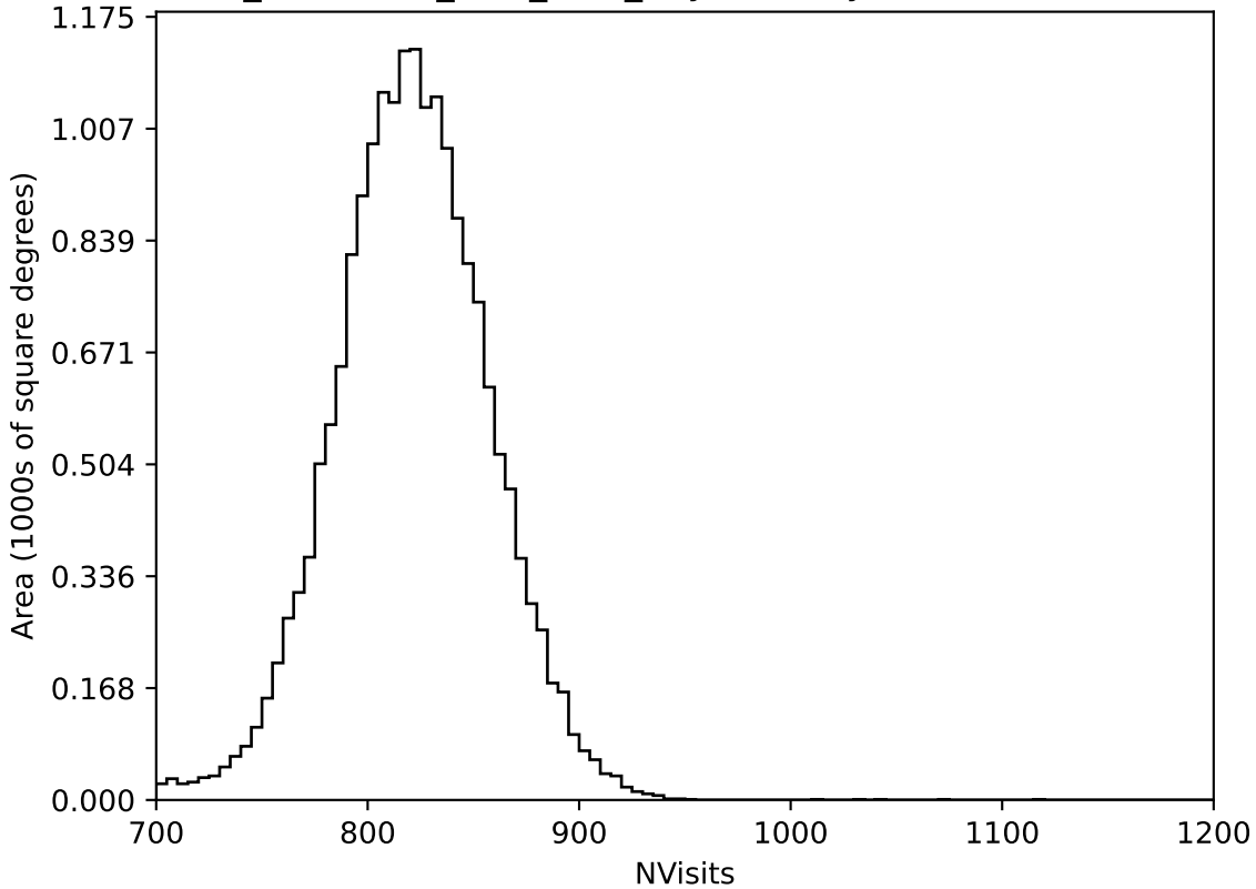
too_combined_s0.5_v3.4_10yrs All sky all bands: NVisits
