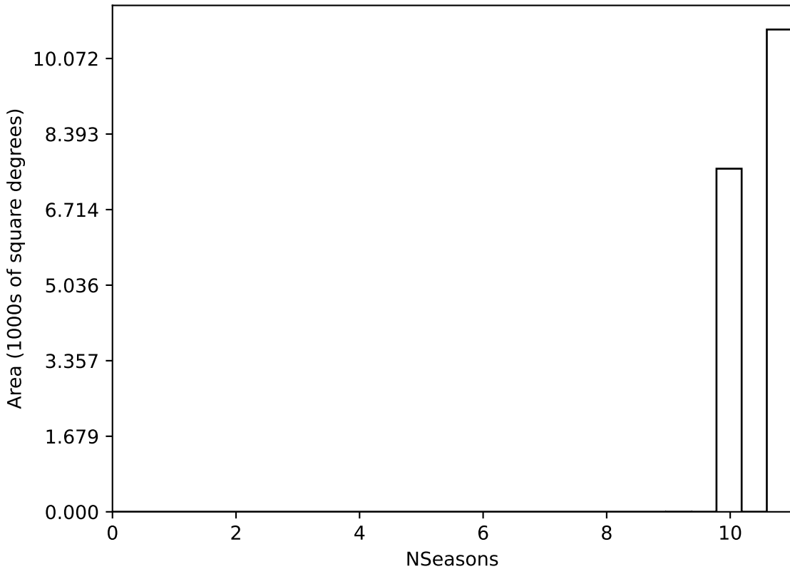
too_combined_s0.5_v3.4_10yrs WFD all bands: NSeasons
