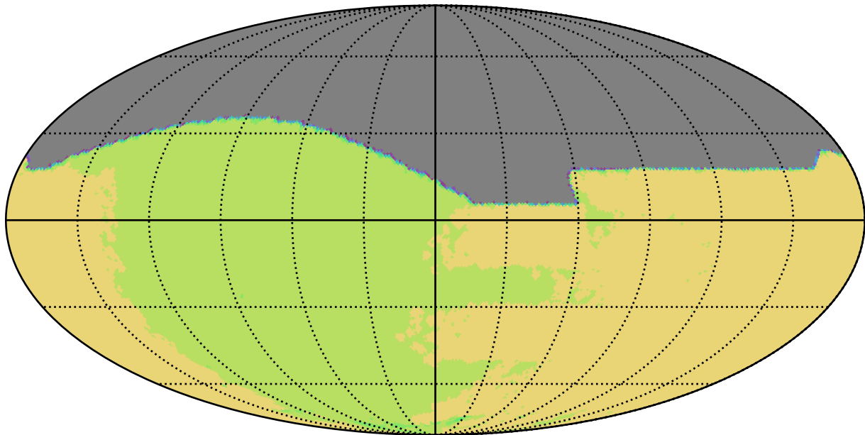
too_combined_s0.5_v3.4_10yrs All sky all bands: NSeasons
