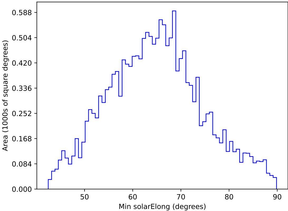
too_combined_s0.5_v3.4_10yrs WFD y band: Min solarElong
