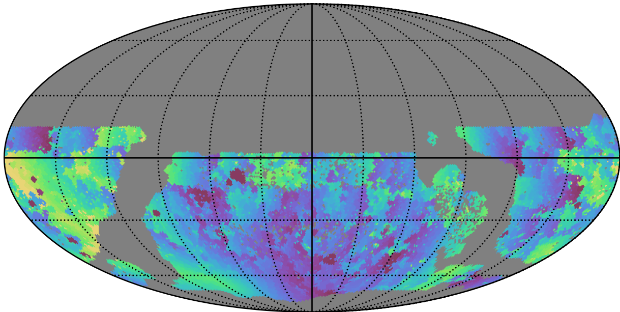
too_combined_s0.5_v3.4_10yrs WFD u band: Min solarElong
