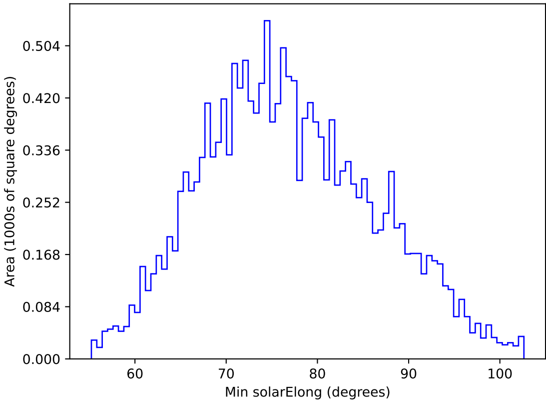
too_combined_s0.5_v3.4_10yrs WFD u band: Min solarElong
