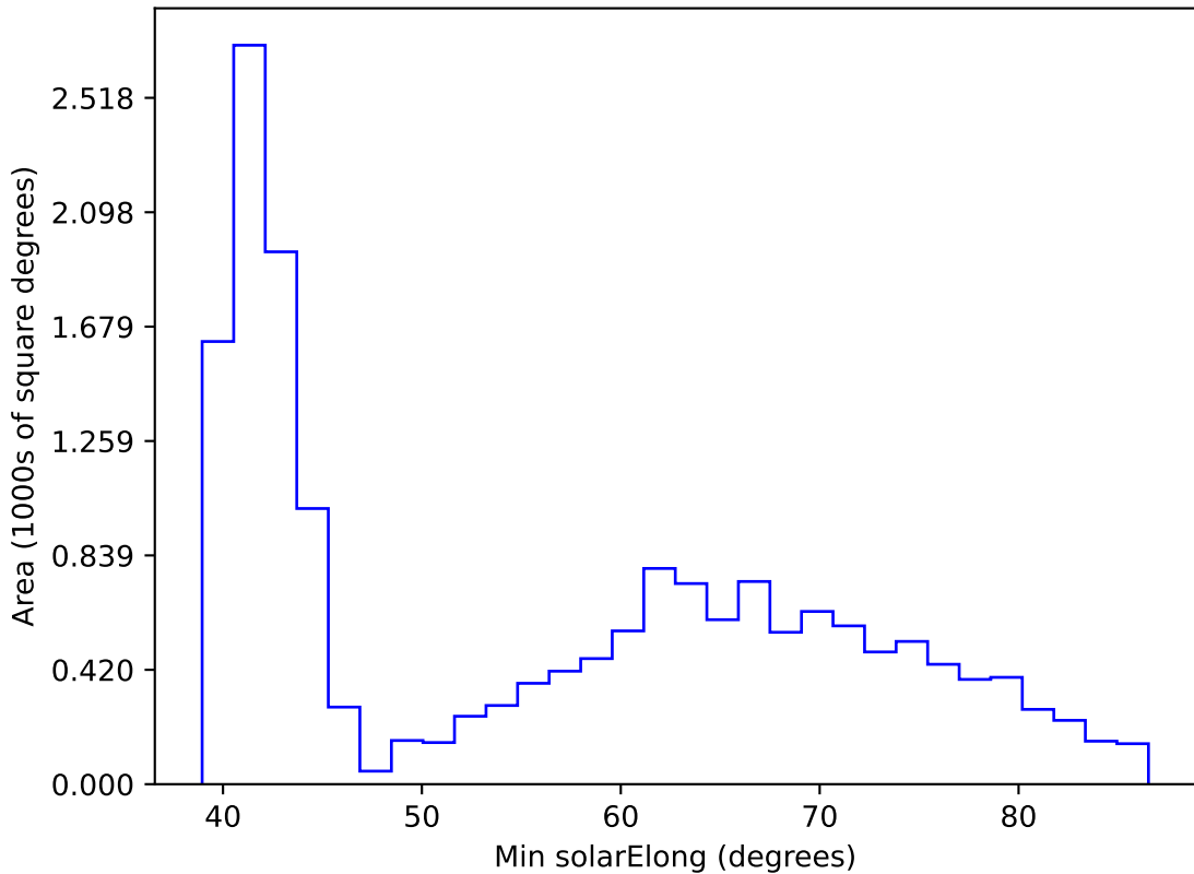
too_combined_s0.5_v3.4_10yrs WFD r band: Min solarElong
