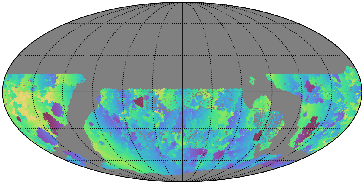
too_combined_s0.5_v3.4_10yrs WFD g band: Min solarElong
