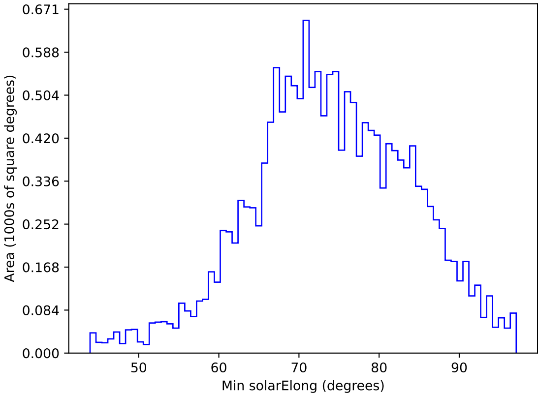
too_combined_s0.5_v3.4_10yrs WFD g band: Min solarElong
