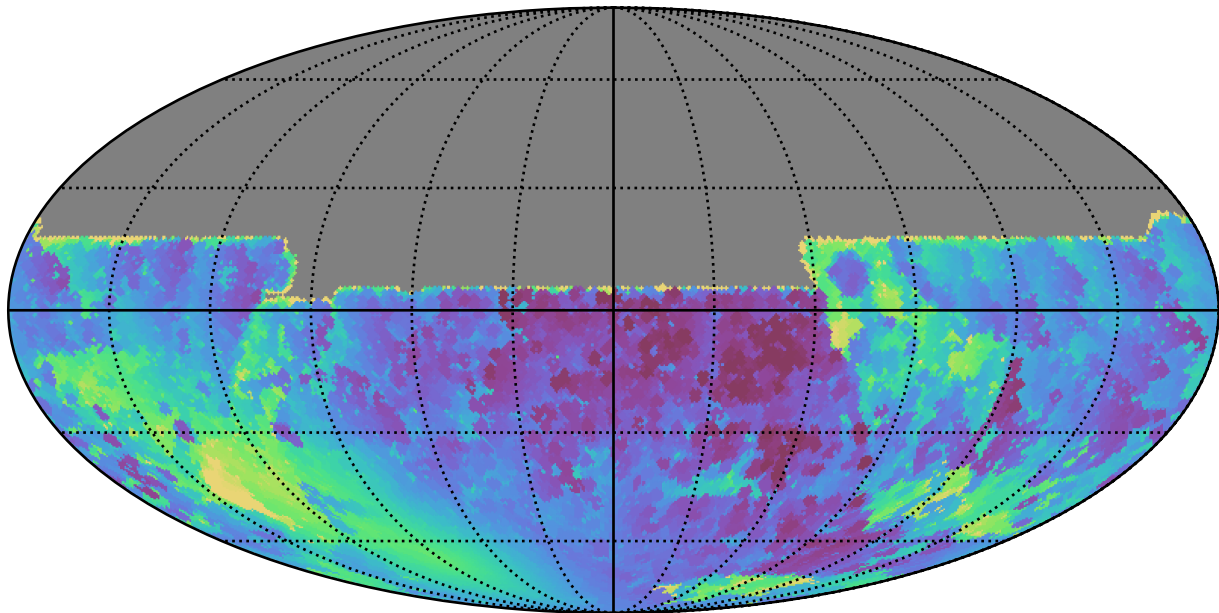
too_combined_s0.5_v3.4_10yrs All sky y band: Min solarElong
