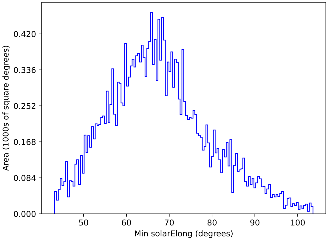
too_combined_s0.5_v3.4_10yrs All sky y band: Min solarElong
