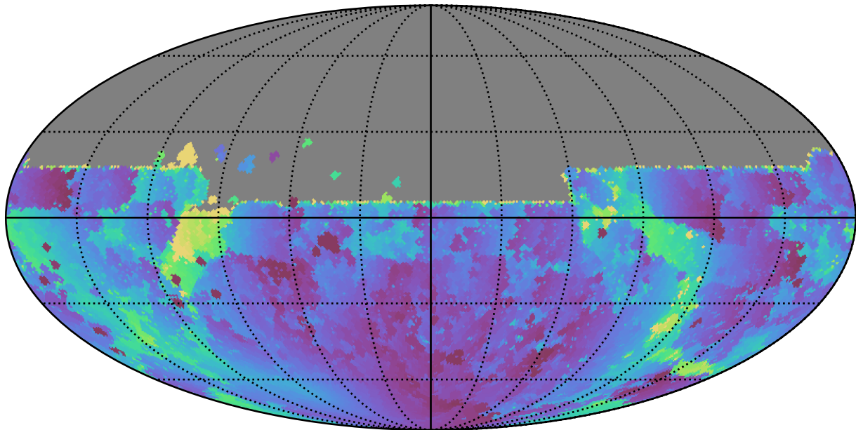
too_combined_s0.5_v3.4_10yrs All sky u band: Min solarElong
