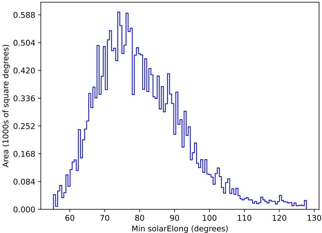
too_combined_s0.5_v3.4_10yrs All sky u band: Min solarElong
