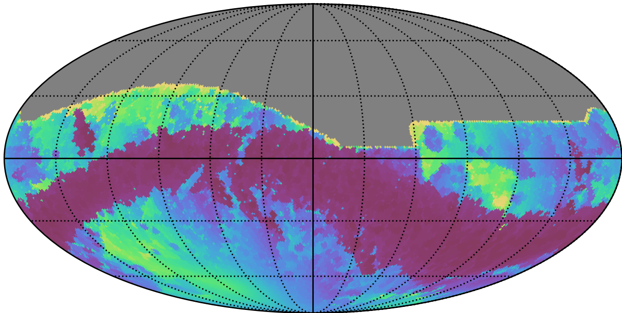
too_combined_s0.5_v3.4_10yrs All sky r band: Min solarElong
