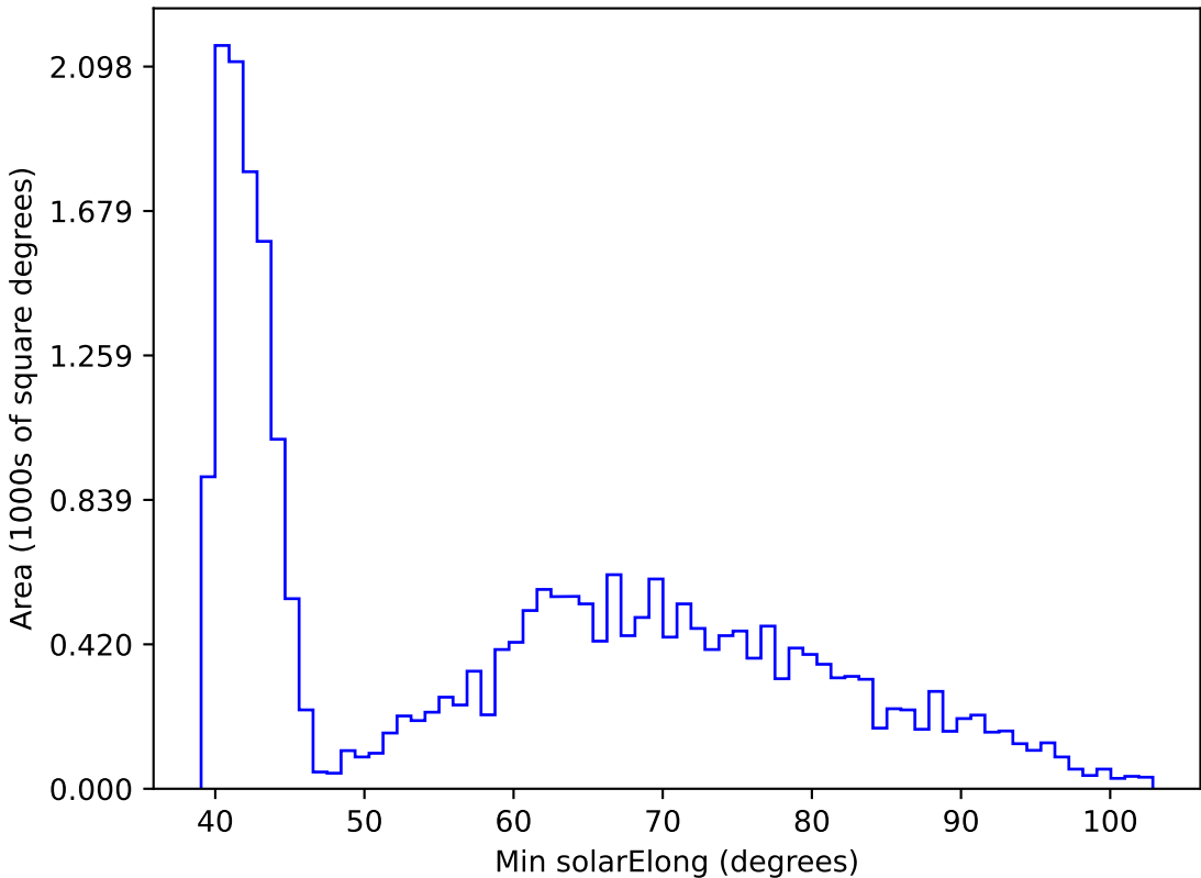
too_combined_s0.5_v3.4_10yrs All sky r band: Min solarElong
