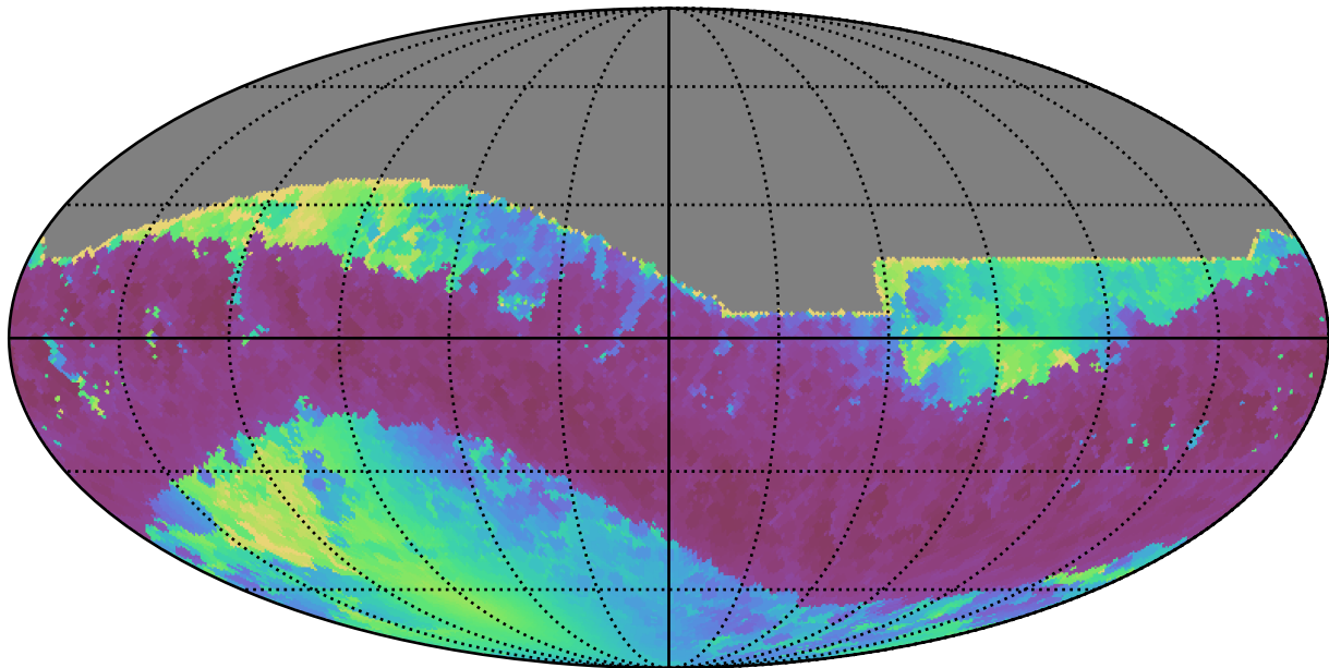
too_combined_s0.5_v3.4_10yrs All sky i band: Min solarElong
