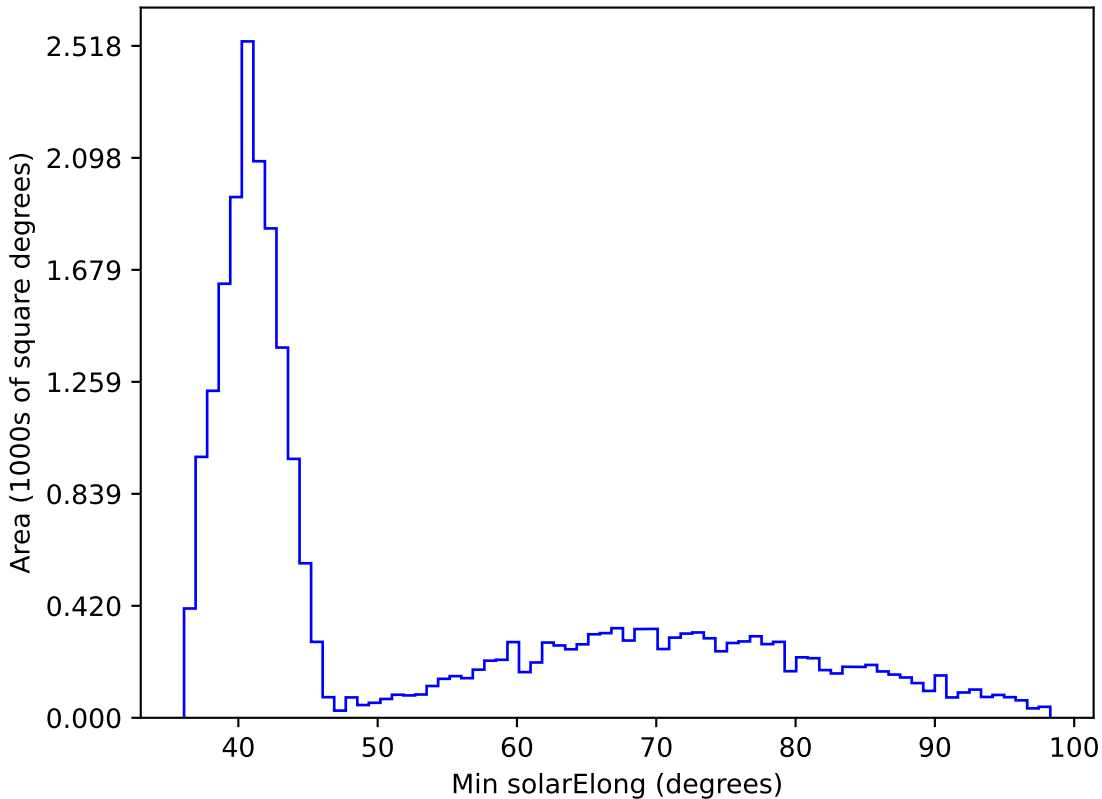
too_combined_s0.5_v3.4_10yrs All sky i band: Min solarElong
