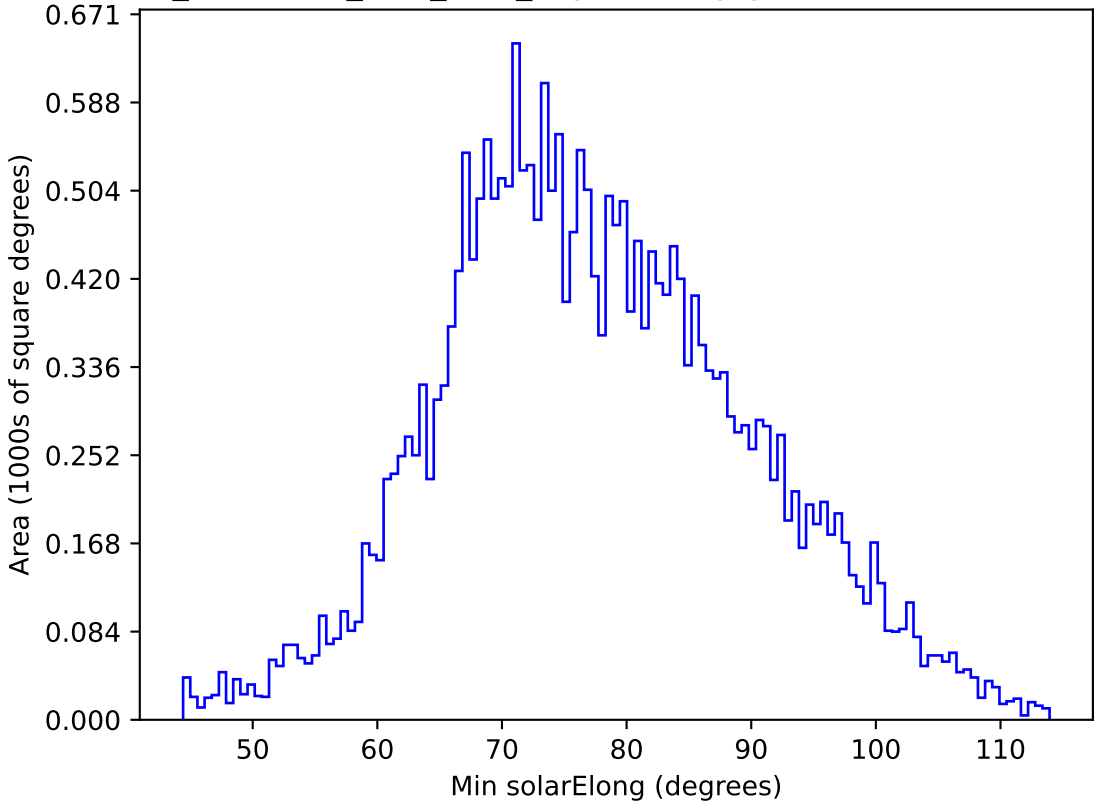
too_combined_s0.5_v3.4_10yrs All sky g band: Min solarElong
