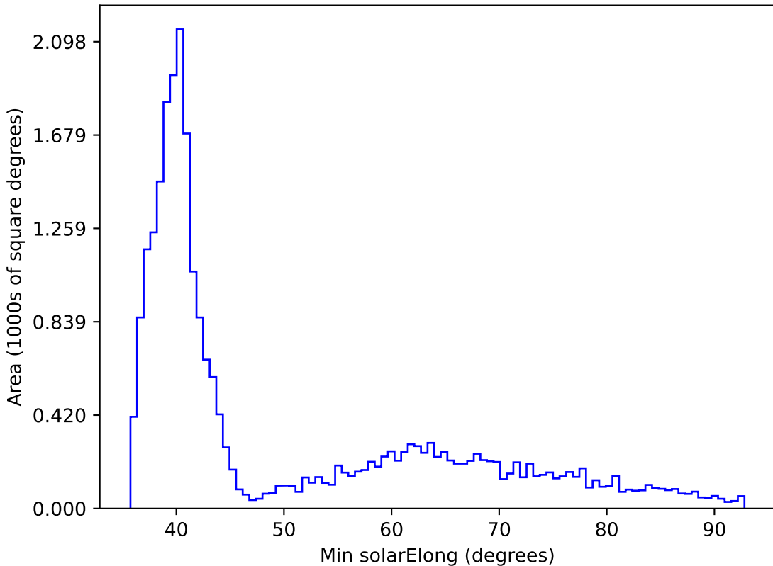
too_combined_s0.5_v3.4_10yrs All sky all bands: Min solarElong
